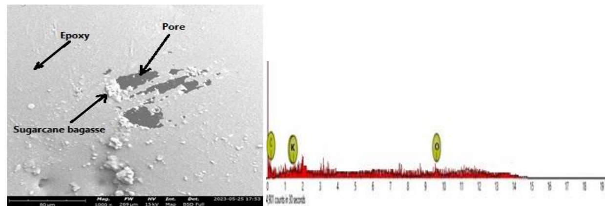
Figure 6: Scanning electron micrograph with EDX spectrum of specimen S2
